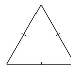
Equilateral triangle three equal sides
