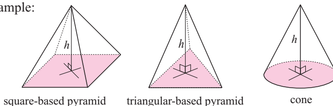
square-based pyramid
